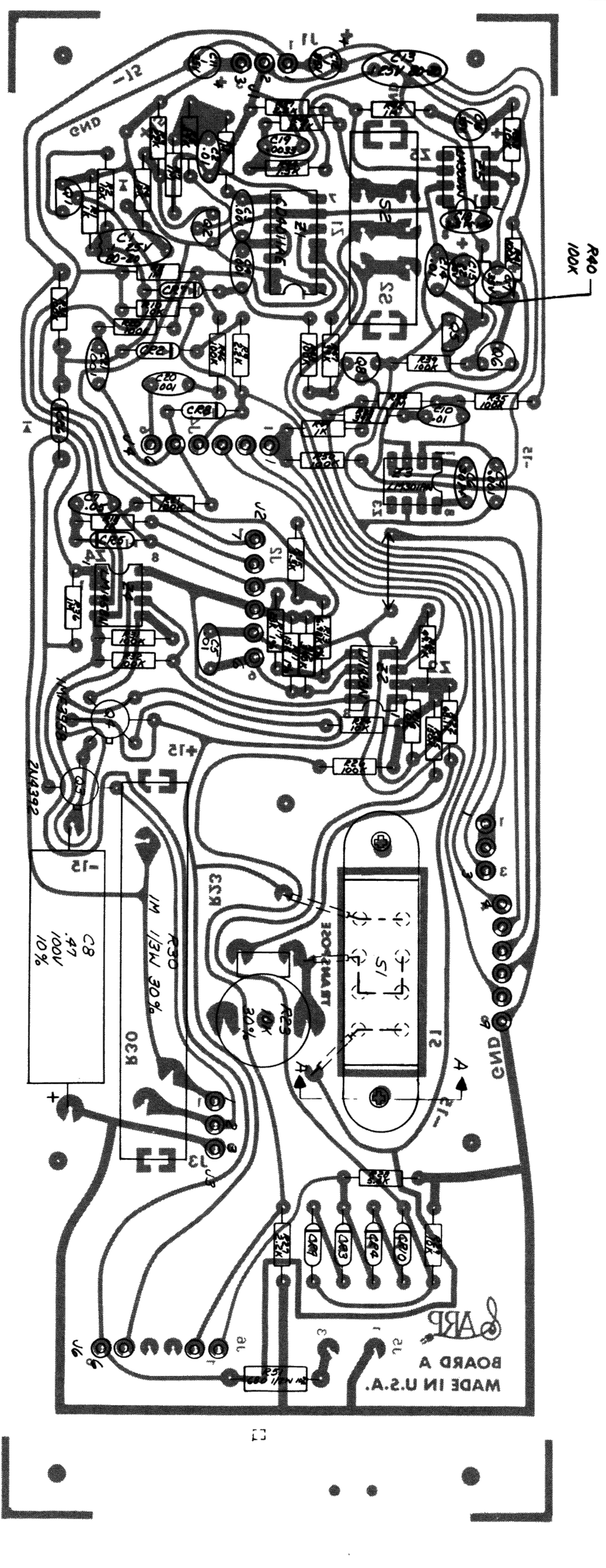
ARP ODYSSEY-2 Model 2810 - 2823 ASSEMBLY Board A-II (with PPC)
