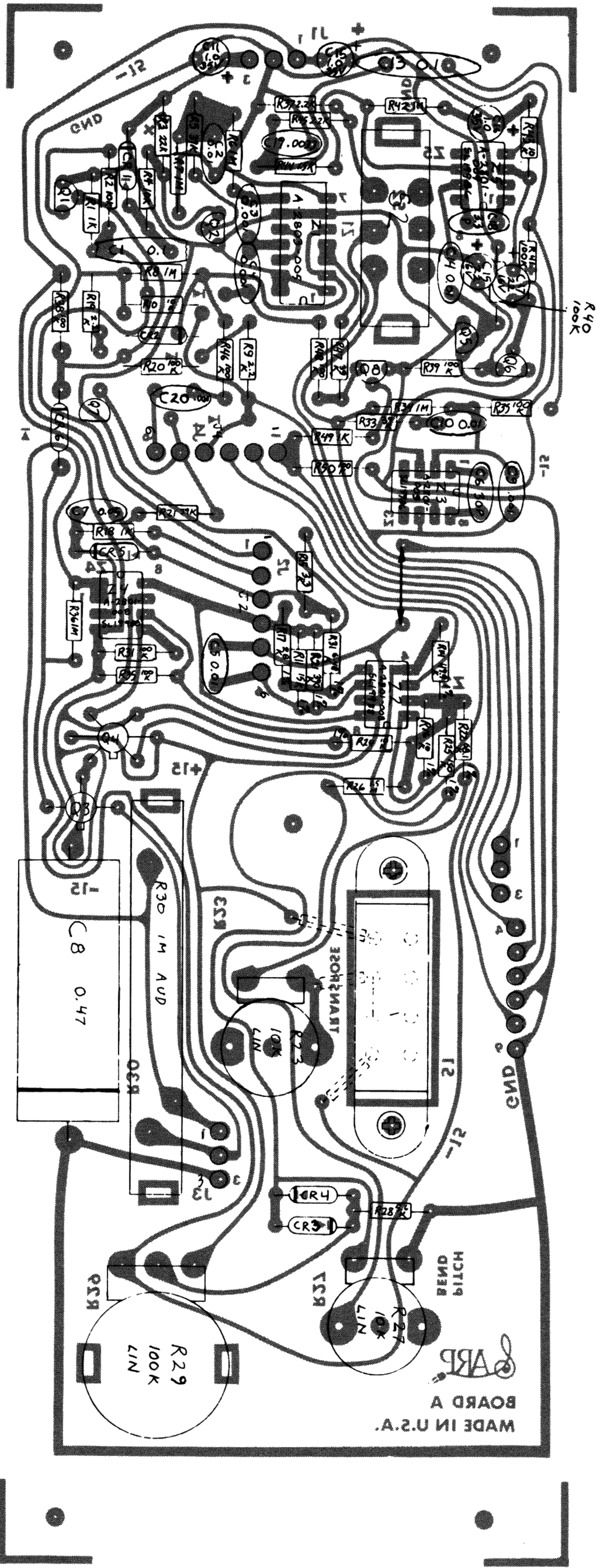
ARP ODYSSEY-2 Model 2810 - 2823 ASSEMBLY Board A-II (without PPC)
