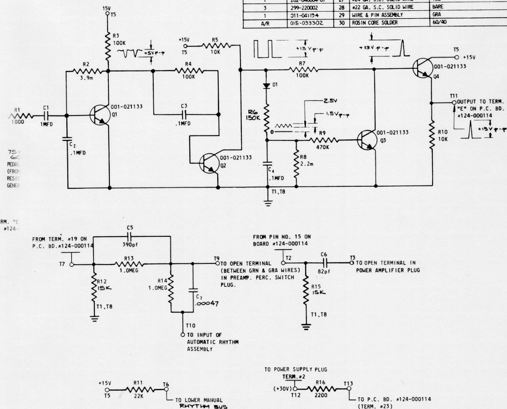
FIGURE 5-8. SCHEMATIC DIAGRAM AND PARTS LAYOUT, PEDAL CONTROL BOARD
