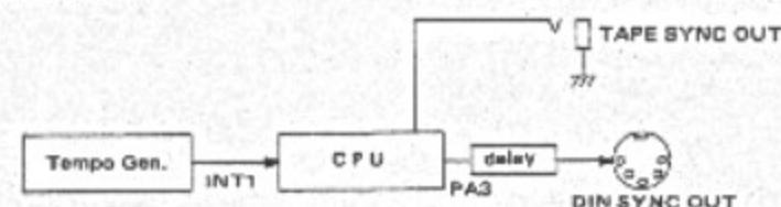
2. Master Mode
