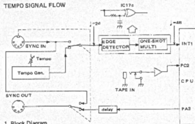
1. Block Diagram
