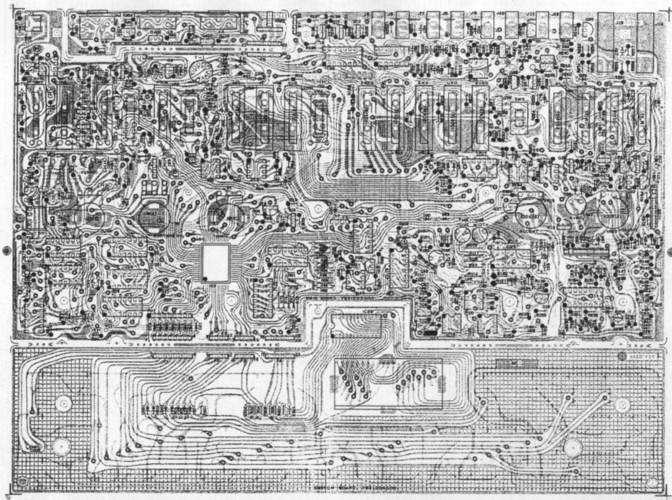
SWITCH BOARD 7931204000 (pcb 2291055600)
