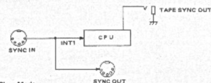
3. Slave Mode
